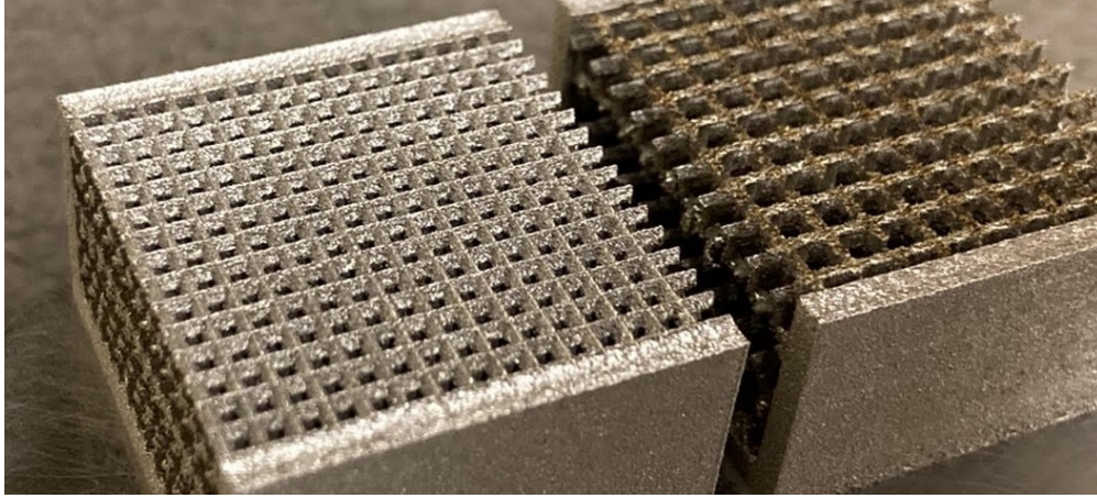
Fig. 6 15 PPI (left) and 10 PPI (right) 316L stainless steel VCMs, created via direct metal laser melting (DMLM) additive manufacturing.
