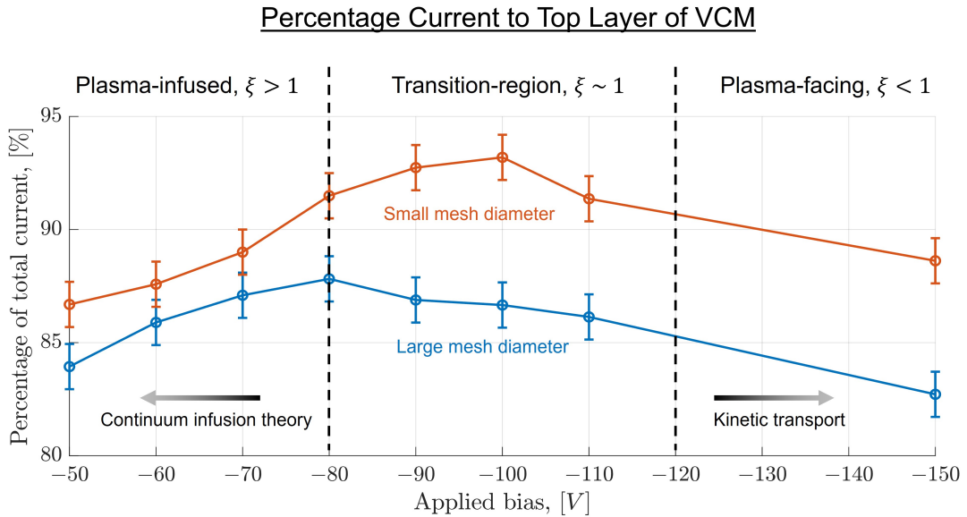
Fig. 4 Percentage of total current collected by the first layer of the stacked mesh structure as a function of applied bias, for two mesh pore sizes of 0.86 mm and 1.9 mm.
