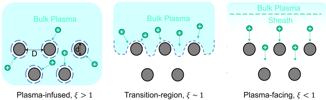
Fig. 2 Three regimes of plasma-material interactions - infused, transitional, and facing. The PMI regime is a function of the plasma properties of temperature and density, as well as the pore diameter of the VCM.
