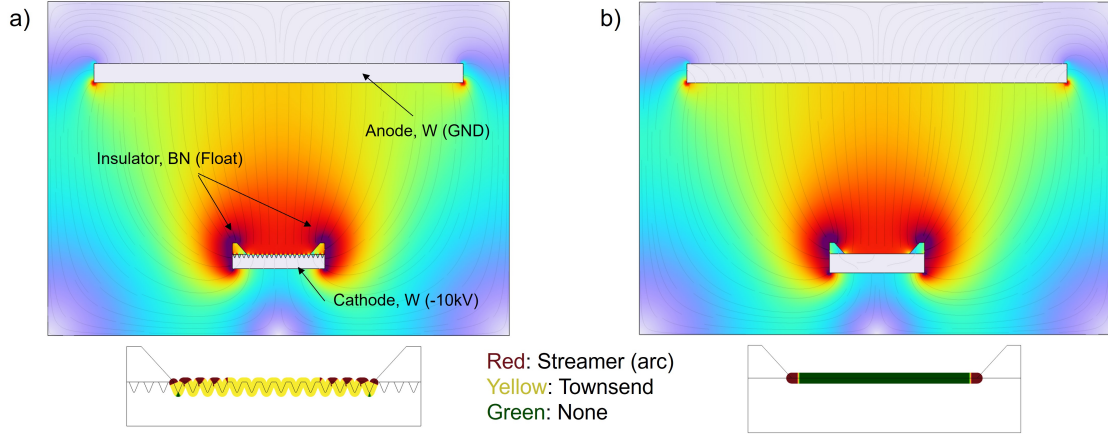
Fig. 11 Breakdown simulation indicating the electric field lines for a) VCM and b) flat samples. VCMs' pointed features lead to enhanced field emission, causing breakdown at a lower potential, relative to flat surfaces. The bottom figures indicate that for arcs on VCMs are more likely to occur at locations other than the triple point junction, leading to the spreading out of the electrical and thermal loads across the face of the sample.
