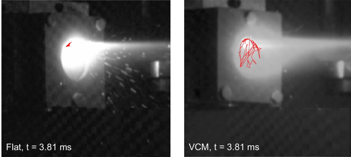
Fig. 10 Differing arcing responses of flat and VCM tungsten samples. A greater quantity of molten ejected material was liberated in the flat sample compared to the VCM. The red traces indicate the motion of the arc path across the samples' face as the arc evolves.
